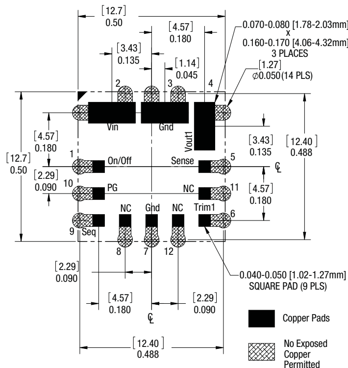
Figure 3. OKL-T/3-W5 Mechanical Outline
