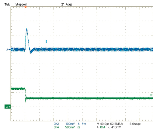
Step Load Transient Response (Vin=5V, Vout=1.5V, Load=0, Iout=3A to 1.5A) Trace 2=Vout, 100 mV/div. Trace 4=Iout, 2.5A/div.
