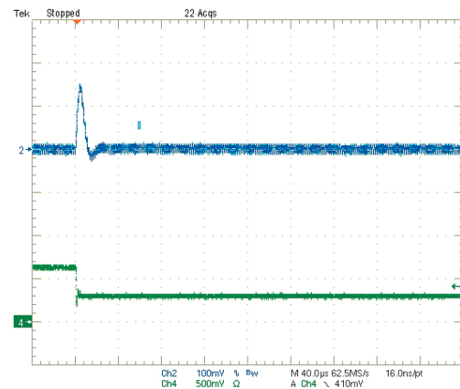
Step Load Transient Response (Vin=5V, Vout=1.8V, Clad=0, Iout=3A to 1.5A) Trace 2=Vout, 100 mV/div. Trace 4=Iout, 2.5A/div.
