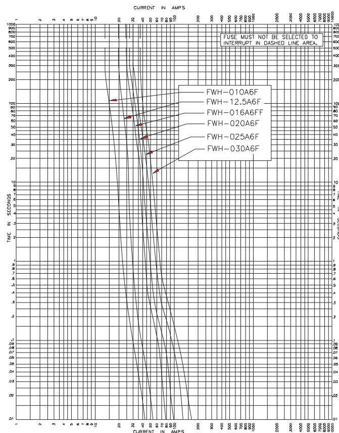
Time-Current Curve
