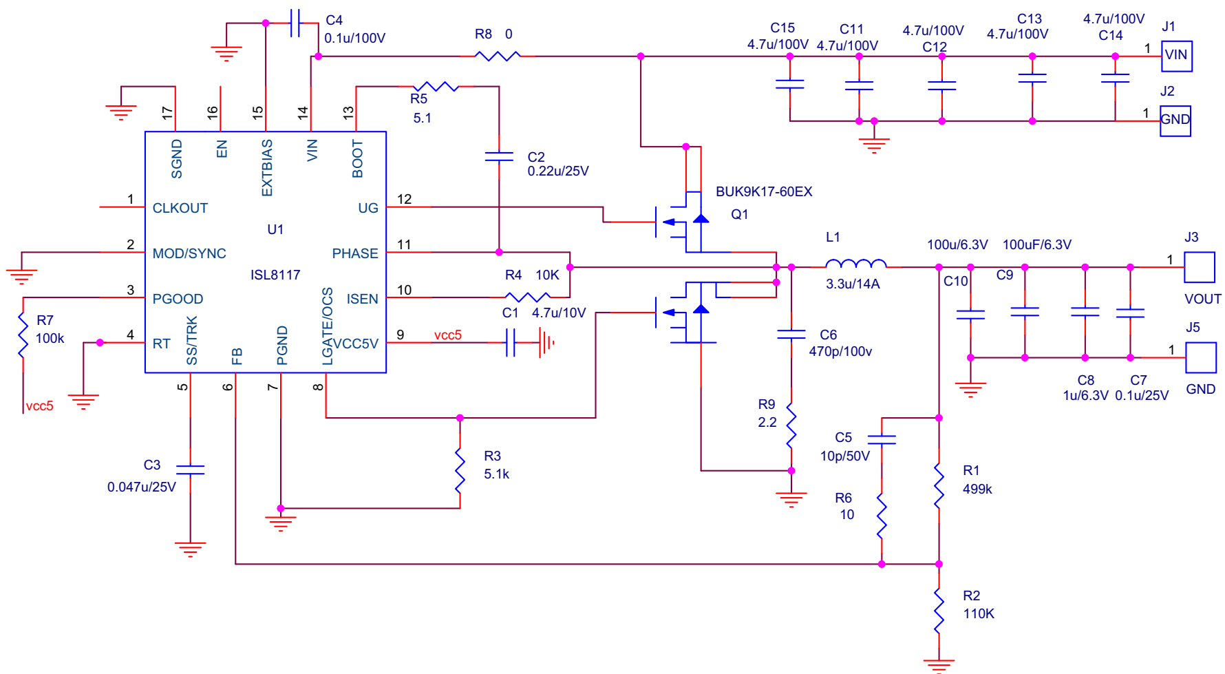
FIGURE 6. ISL8117DEM03Z SCHEMATIC
