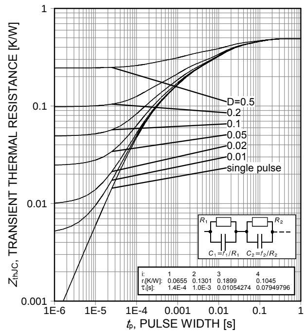
Figure 18. IGBT transient thermal resistance ( D=t_p/T )
