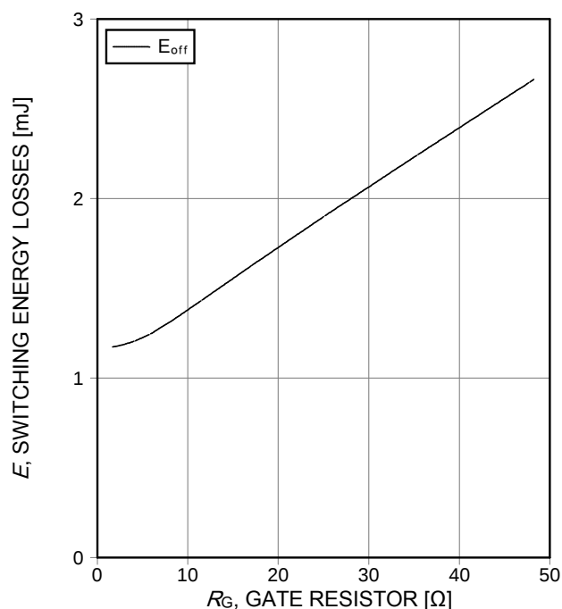
Figure 14. Typical switching energy losses as a function of gate resistor (inductive load, T_j=175^\circ\text{C} , V_{CE}=400\text{V} , I_c=40\text{A} , V_{GE}=15/0\text{V} , Dynamic test circuit in Figure E)
