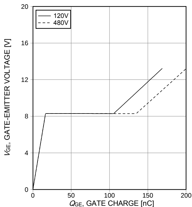
Figure 16. Typical gate charge ( I_c=40\text{A} )
