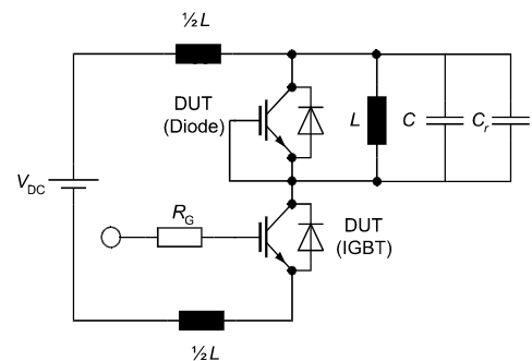
Figure E. Dynamic test circuit Leakage inductance L = 180\text{nH} , Stray capacitor C_g = 40\text{pF} , Relief capacitor C_r = 1\text{nF} (only for ZVT switching)
