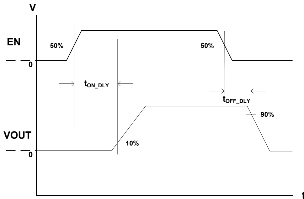
Figure 2. Turn-On/Off Delay
