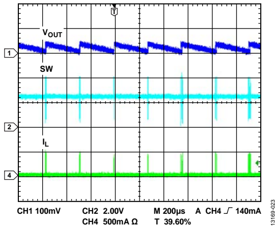
Figure 23. Steady Waveform of Hysteresis Mode, I LOAD = 1 mA (I L is the Inductor Current)
