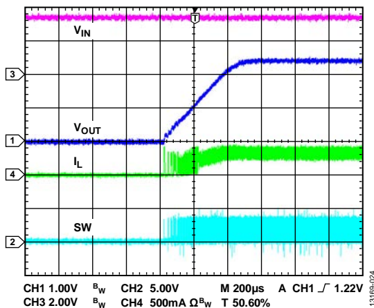
Figure 24. Soft Start, I LOAD = 300 mA
