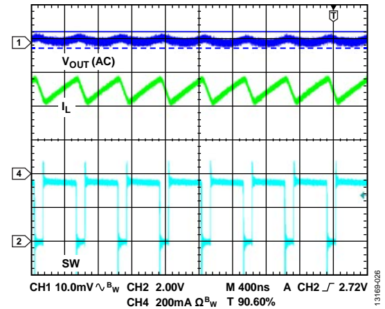
Figure 26. Steady Waveform of PWM Mode, I LOAD = 300 mA
