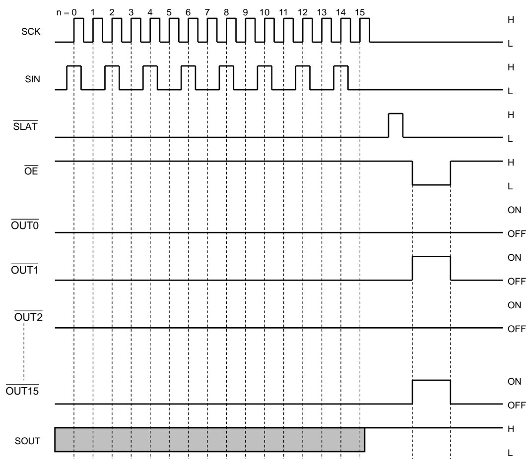
Timing Diagram
