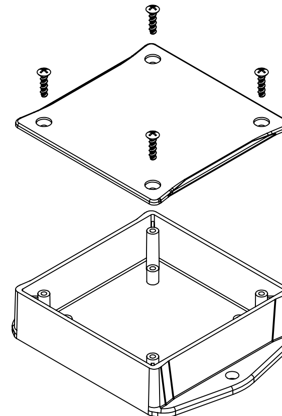
—PC BOARD MOUNTING BOSSES ACCEPT #4 x 1/4" LG THREAD FORMING SCREWS (NOT SUPPLIED)
