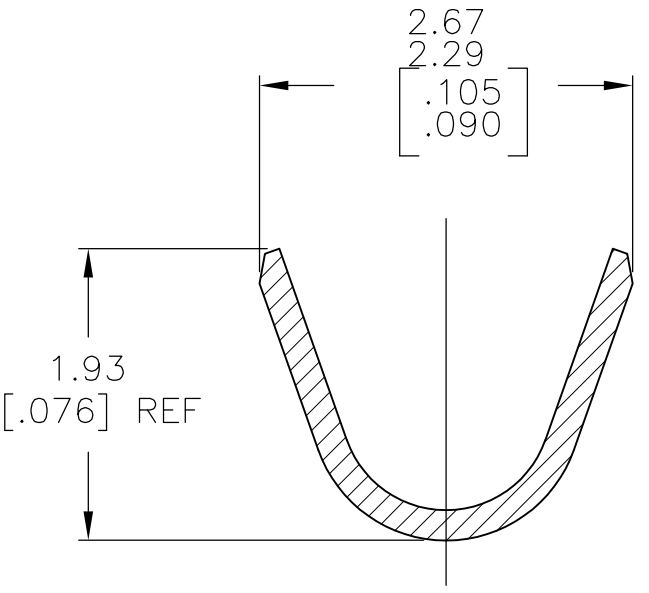
SECTION B-B SCALE 20:1
