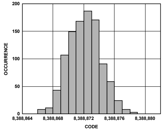
Figure 12. Noise Distribution Histogram ( V_{REF} = AV_{DD} = 5\text{ V} , Output Data Rate = 42.1 Hz (FS[9:0] = 6, Average by 16), Gain = 1, Chop Disabled, Sinc 4 Filter)
