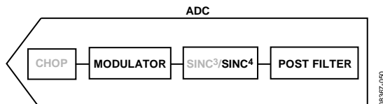
Figure 54. Fast Settling Mode, Sinc 4 Filter
