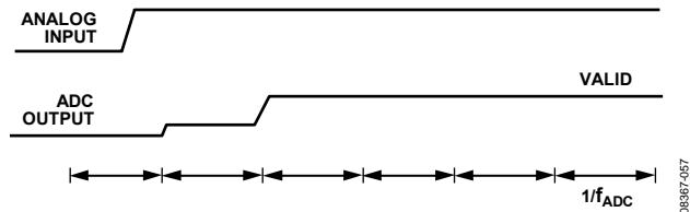
Figure 63. Step Change on Analog Input, Sinc 3 Filter
