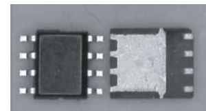
Standard SO-8 PowerPAK SO-8
