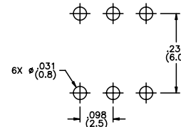
P.C. board layout
