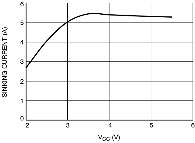
Figure 10. Maximum Sinking Current vs. V_{CC} ( V_{DDQ} = PV_{CC} = 1.8\text{ V} )
