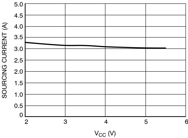
Figure 12. Maximum Sourcing Current vs. V_{CC} ( V_{DDQ} = PV_{CC} = 2.5\text{ V} )
