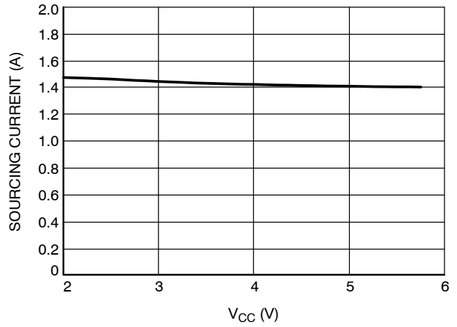
Figure 11. Maximum Sourcing Current vs. V_{CC} ( V_{DDQ} = 2.5\text{ V} , PV_{CC} = 1.8\text{ V} )
