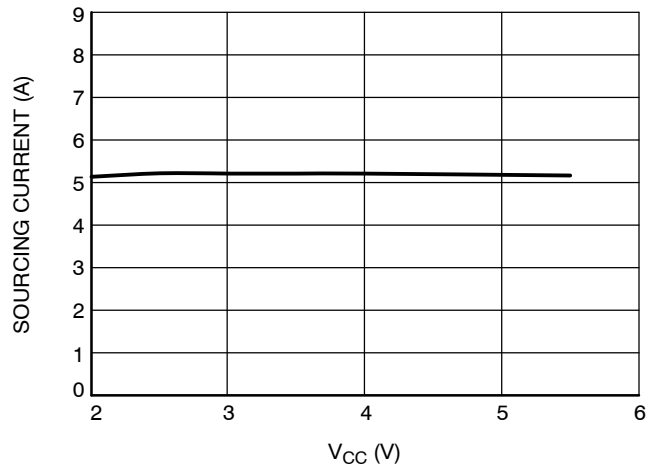
Figure 13. Maximum Sourcing Current vs. V_{CC} ( V_{DDQ} = 2.5\text{ V} , PV_{CC} = 3.3\text{ V} )
