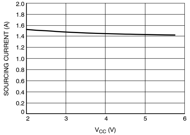
Figure 9. Maximum Sourcing Current vs. V_{CC} ( V_{DDQ} = PV_{CC} = 1.8\text{ V} )
