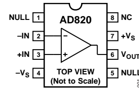
NC = NO CONNECT
