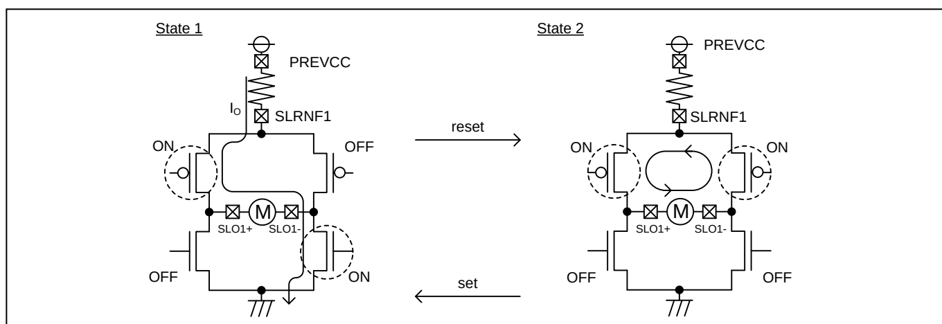
Figure 15. Current Paths in Set [State 1] and Reset [State 2]
