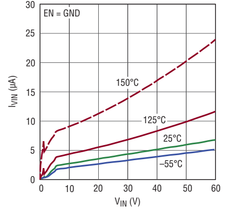
Input Shutdown Current vs Input Voltage
