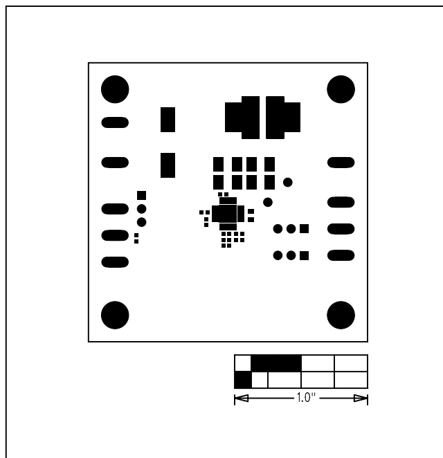
Figure 17. MAX17504 3.3V Output EV Kit Component Placement Guide—Top Solder Mask
