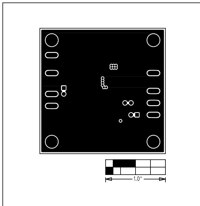
Figure 14. MAX17504 3.3V Output EV Kit PCB Layout—Inner Layer 1
