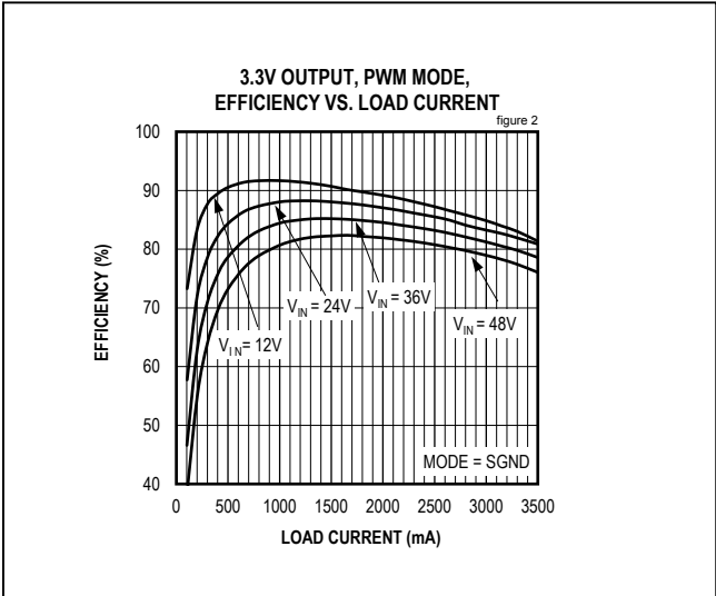
Figure 2. MAX17504 3.3V Output Efficiency (PWM Mode)
