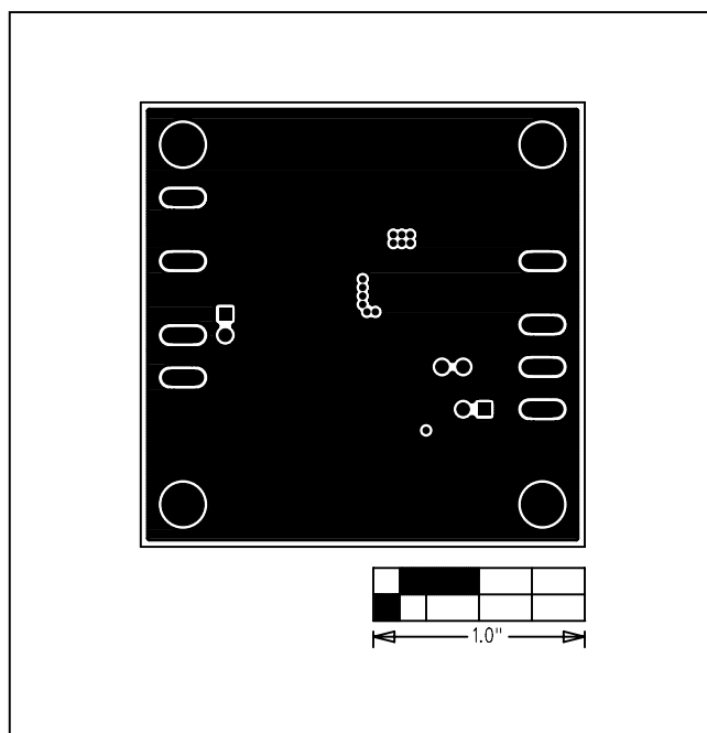
Figure 15. MAX17504 3.3V Output EV Kit PCB Layout—Inner Layer 2
