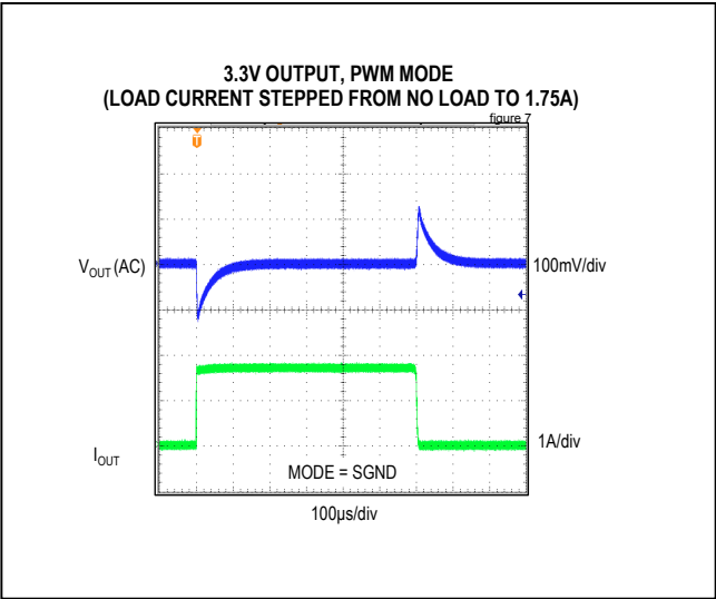
Figure 7. MAX17504 3.3V Output, No Load to 1.75A Load Transient (PWM Mode)
