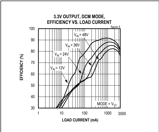
Figure 5. MAX17504 3.3V Output Efficiency (DCM Mode)
