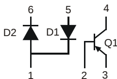
Device Schematic
