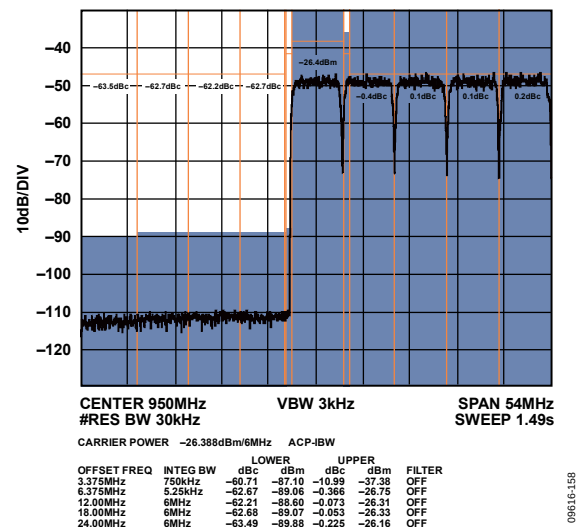
Figure 59. High Band Narrow-Band ACLR
