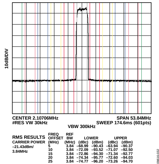
Figure 109. Typical Single-Carrier WCDMA ACLR Performance at 2.1 GHz, f_{DAC} = 2457.6 MSPS (Second Nyquist Zone)
