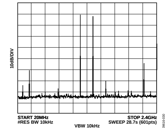
Figure 110. Single-Tone Spectrum in Mix-Mode at f_{OUT} = 1.31 GHz, f_{DAC} = 2.4 GSPS
