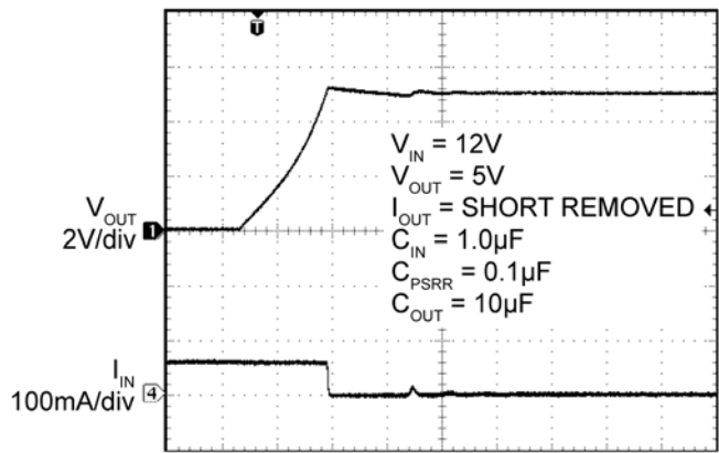
Time (400µs/div)
