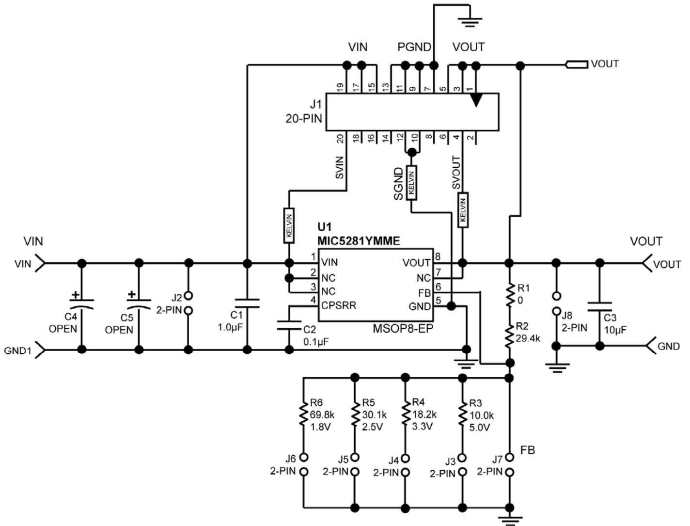
MIC5281 Evaluation Board Schematic
