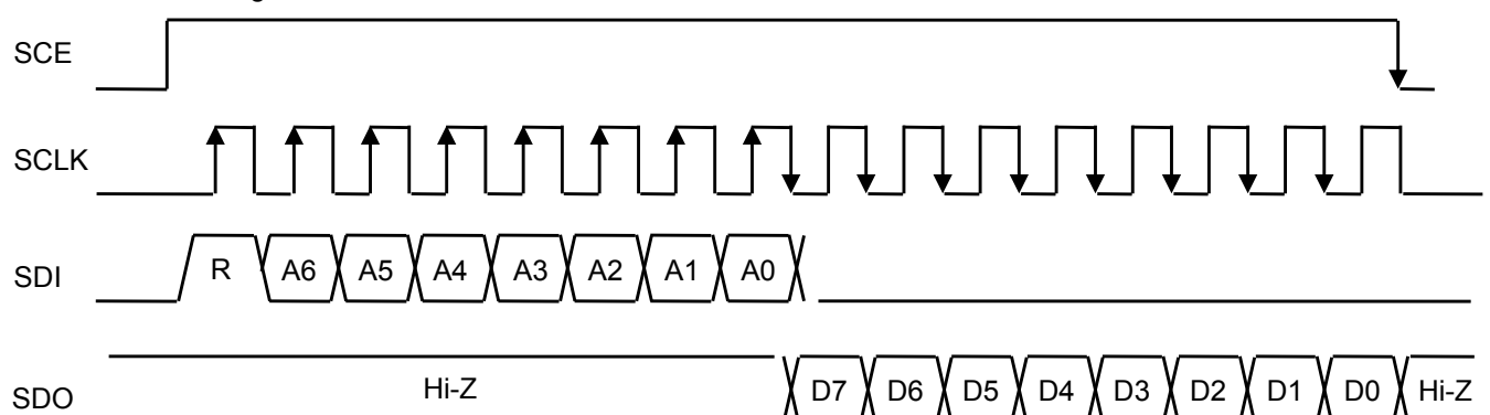
Transmission timing
