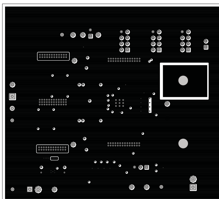
Figure 21. TPS51727EVM Internal Layer 5, Top View
