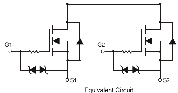
Equivalent Circuit
