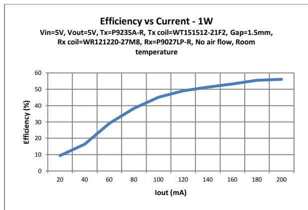
Figure 4. Typical Performance Characteristics – 1W
