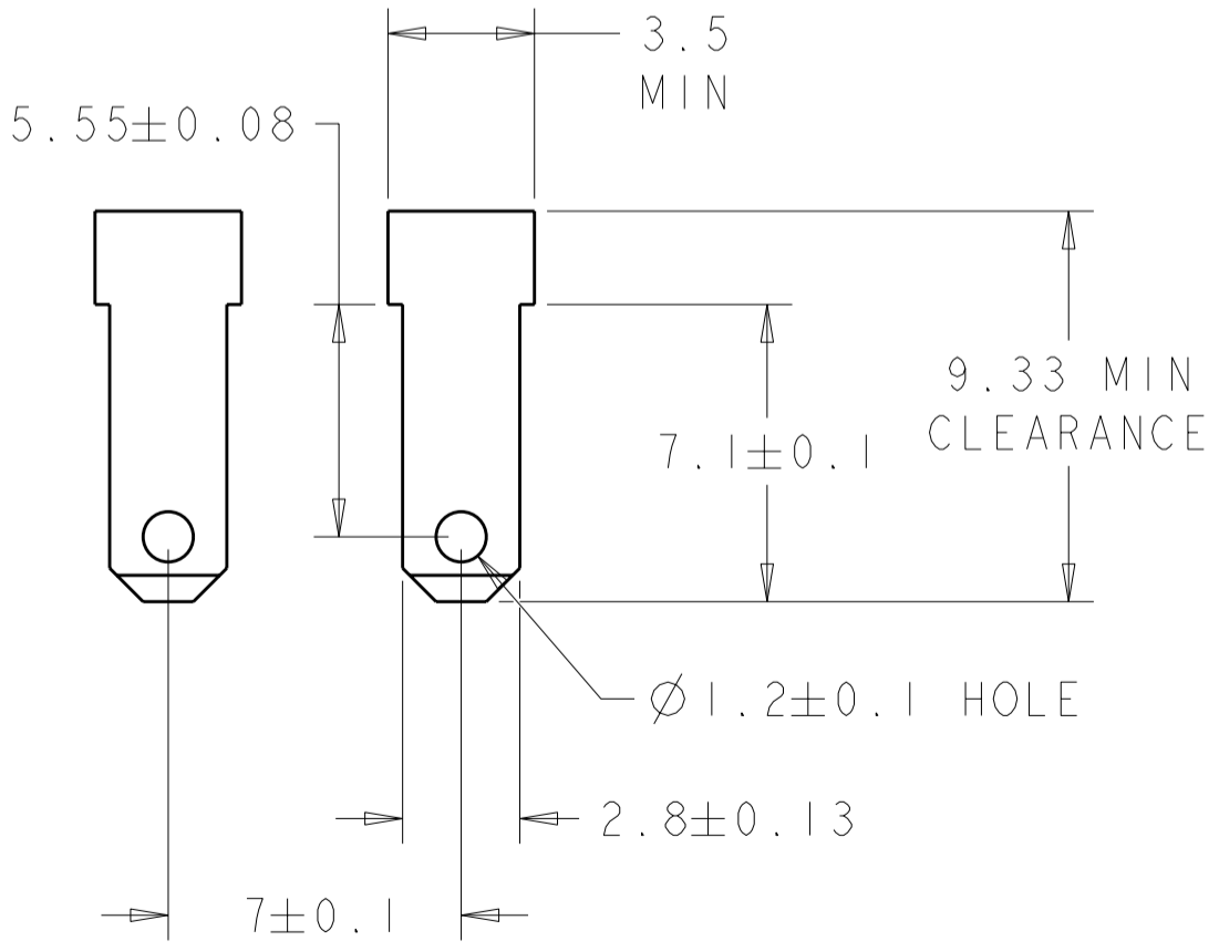
SCALE 5:1 MATING TAB DIMENSIONS
