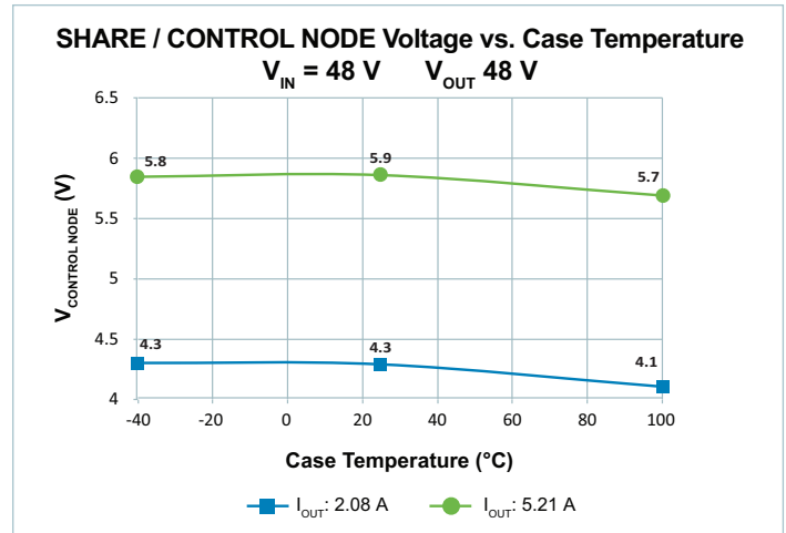
Figure 17 — Typical SHARE / CONTROL NODE Voltage vs. T_{\text{CASE}} and I_{\text{OUT}} ; V_{\text{IN}} = 48.0\text{ V} , V_{\text{OUT}} = 53.0\text{ V}
