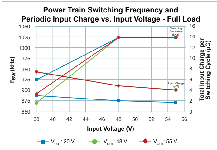
Figure 14 — Typical Power Train Switching Frequency and Periodic Input Charge vs. V_{\text{IN}} , V_{\text{OUT}} , I_{\text{OUT}} = 4.72\text{ A}
