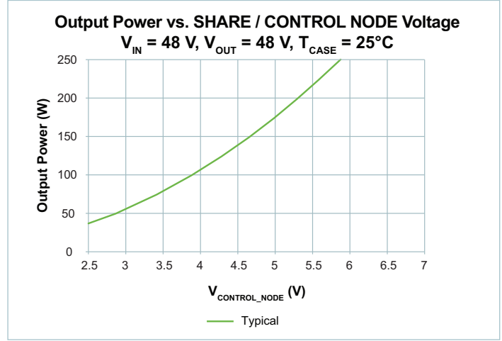
Figure 16 — Output Power vs. SHARE / CONTROL NODE Voltage; V_{\text{IN}} = 48.0\text{ V} , V_{\text{OUT}} = 53.0\text{ V} , T_{\text{CASE}} = 25^\circ\text{C}
