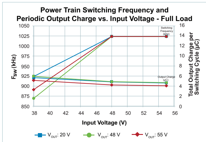
Figure 15 — Typical Power Train Switching Frequency and Periodic Output Charge vs. V_{\text{IN}} , V_{\text{OUT}} , I_{\text{OUT}} = 4.72\text{ A}
