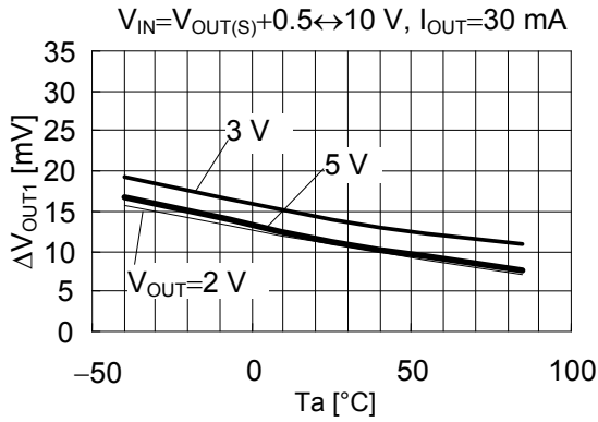
S-814A20A/S-814A30A/S-814A50A
