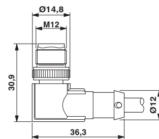
Dimensioned drawing
