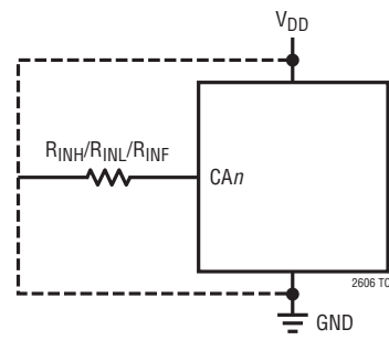
Test Circuit 2
