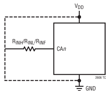
Test Circuit 2
