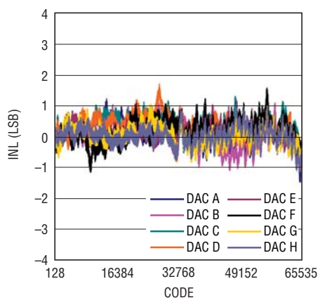
INL vs Code (LTC2657-16)
