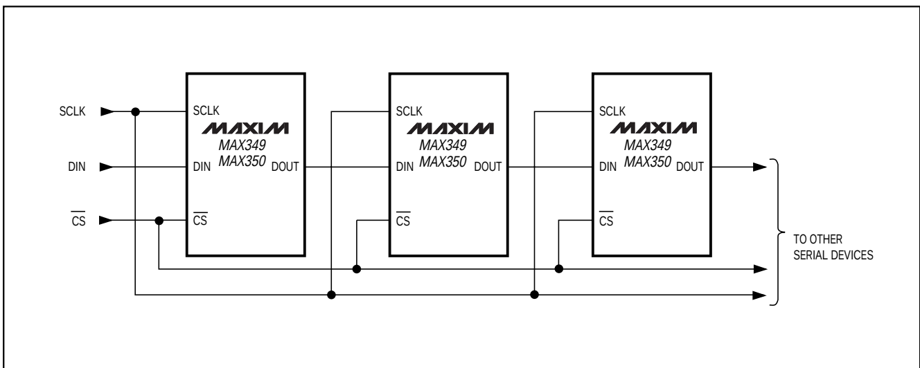
Figure 5. Daisy-Chained Connection
