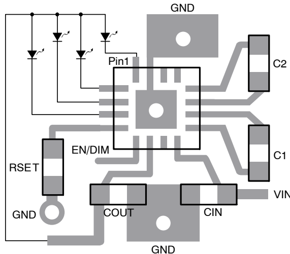
Figure 27. Recommended Layout
