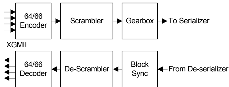
Figure 21: 10GBASE-R PCS
