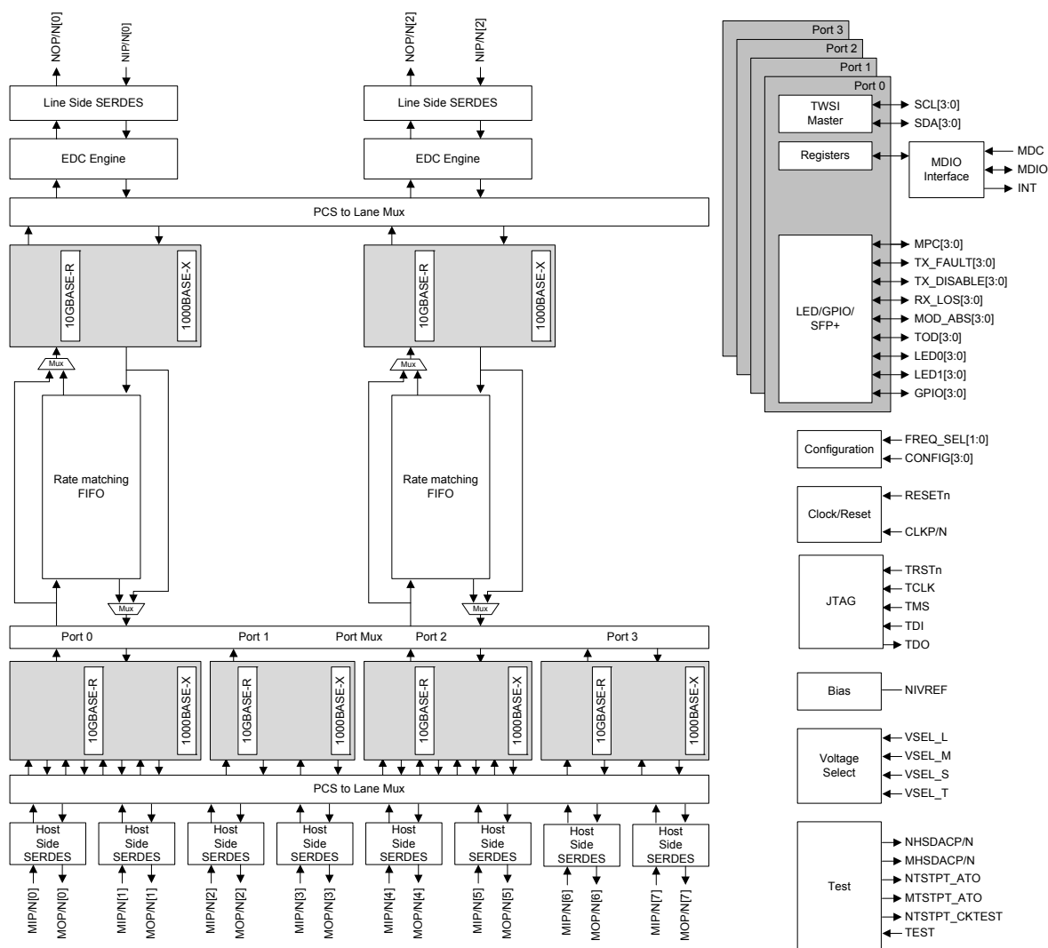
Figure 1: 88X2222 Device Functional Block Diagram
