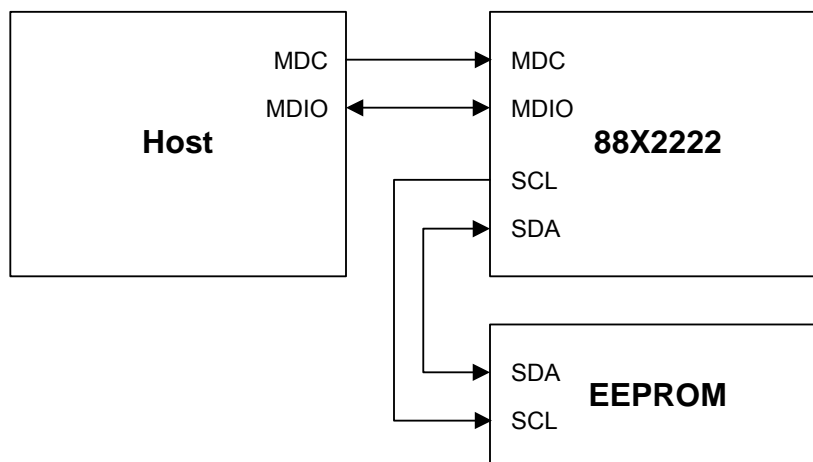
Figure 11: MDC/MDIO Bridging
