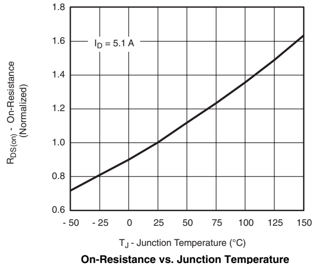
I_D = 5.1 \text{ A} On-Resistance vs. Junction Temperature
