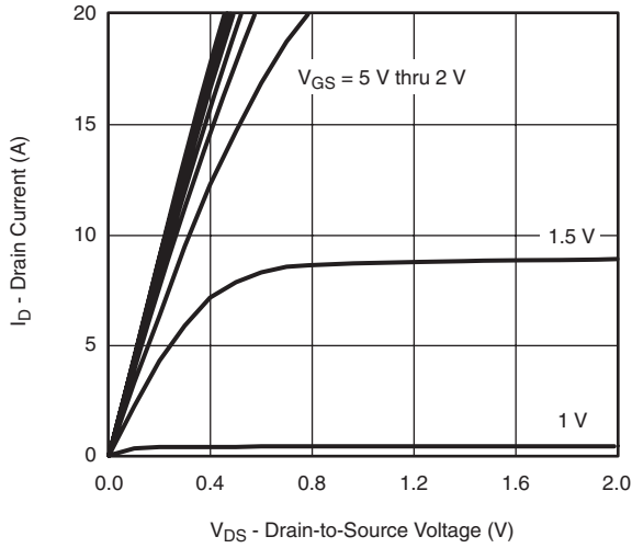
V_{GS} = 5 \text{ V thru } 2 \text{ V} Output Characteristics
