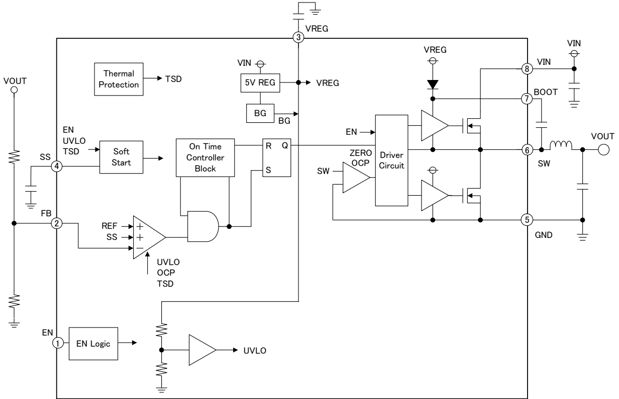
Figure 3. Block Diagram
