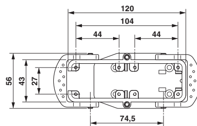
Dimensional drawing, a = 120 mm
