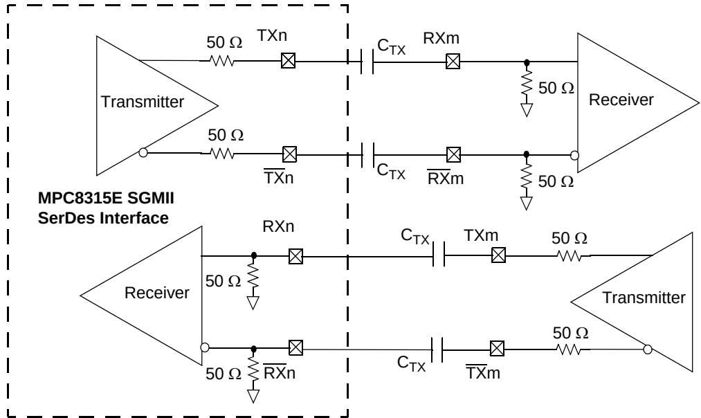
Figure 17. 4-Wire AC-Coupled SGMII Serial Link Connection Example
