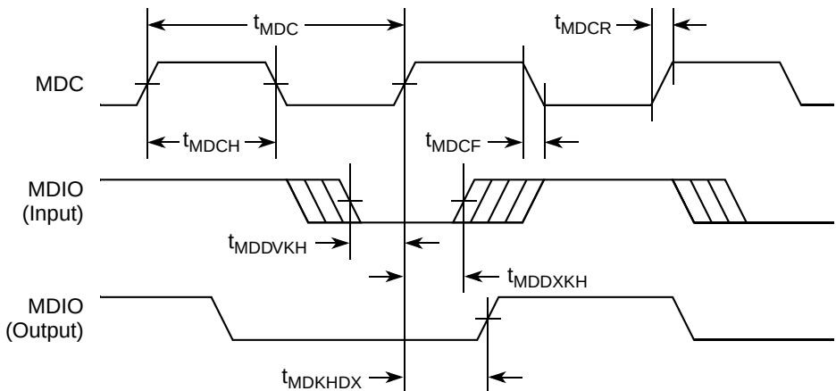
Figure 16. MII Management Interface Timing Diagram
