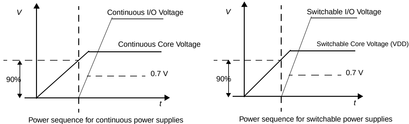
Figure 3. Power-Up Sequencing
