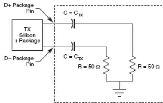
Figure 20. SGMII AC Test/Masurement Load
