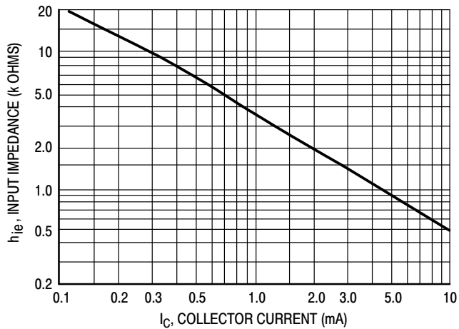
Figure 14. Input Impedance
