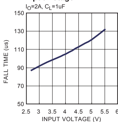
Fall Time vs. Input Votage
