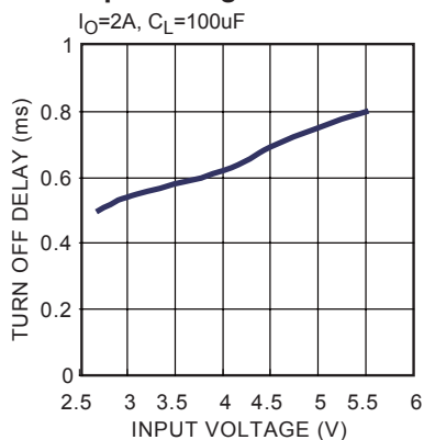
Turn off Delay vs. Input Votage
