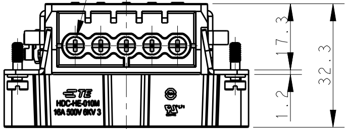
10X M3 SCREW, RECOMMENDED TIGHTENING TORQUE 0.5Nm 10X M3螺丝, 推荐锁紧力矩0.5Nm
