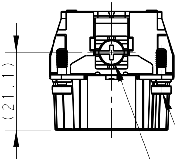
4X M3 SCREW, RECOMMENDED TIGHTENING TORQUE 0.5Nm 4X M3螺丝, 推荐锁紧力矩0.5Nm
