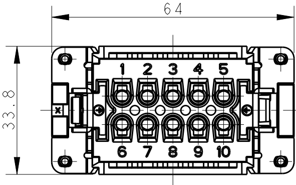
10X M3 SCREW, RECOMMENDED TIGHTENING TORQUE 0.5Nm 10X M3螺丝, 推荐锁紧力矩0.5Nm
