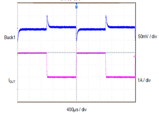
Load Transient Buck1- Vout=3.3V 1A to 3A
