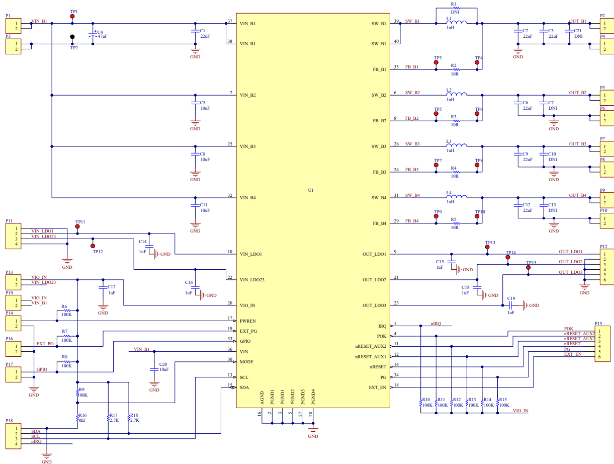
Figure 5 – ACT8870EVK1-102 Schematic
