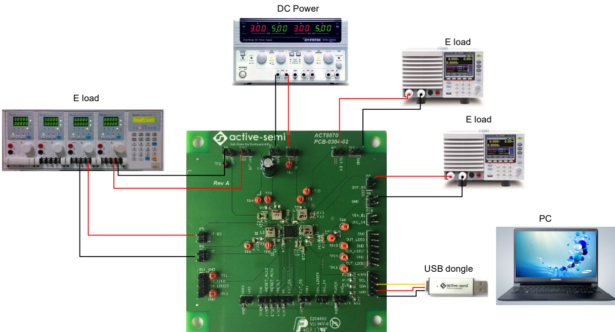
Figure 2 – EVK Setup
