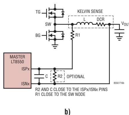
Figure 16. Inductor Current Sense Filter
