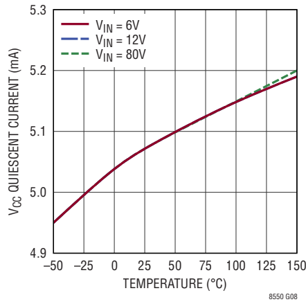
V CC Quiescent Current vs Temperature, Not Switching
