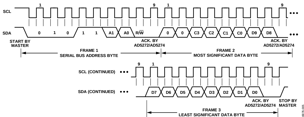
Figure 43. Write Command
