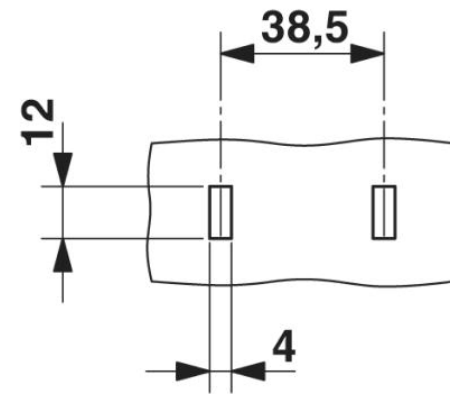
Punching template
